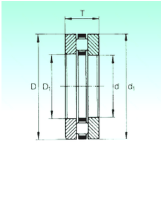
81252-M Bearing 2D drawings and 3D CAD models
